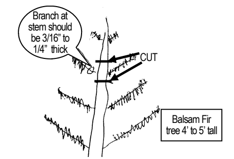
Fig. 1 Where stem is 3/4" to 1" thick, cut it 1" below the branch and 3" above the branch.
